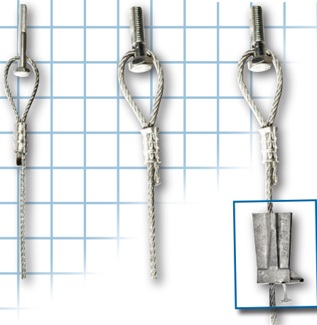
1/4 Threaded Bolt 3/8 Threaded Bolt 3/8 Threaded Bolt with Zip-Clip
